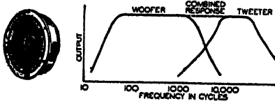
Tweeter loudspeaker—example and response curve.
